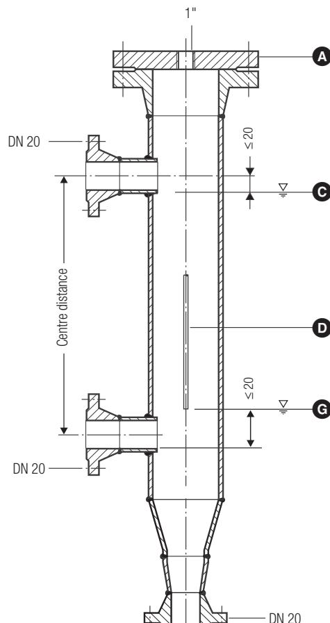
Fig. 4 External measuring pot
