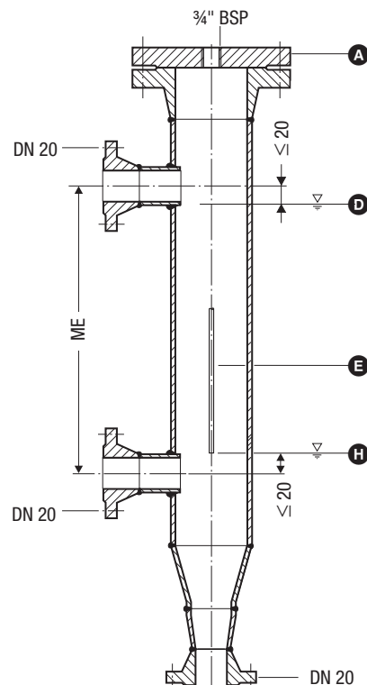
Fig. 3 External measuring pot
