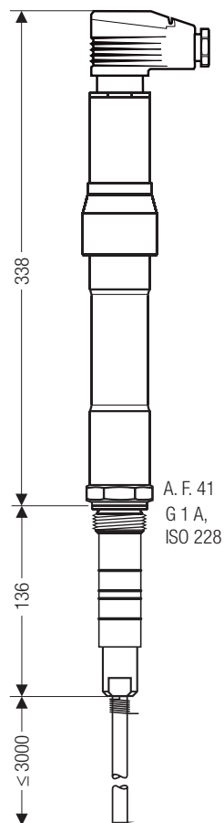
Fig. 2 NRG 111-50 with four-pole connector
