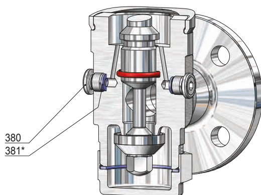
Manometer connection G 1/4
