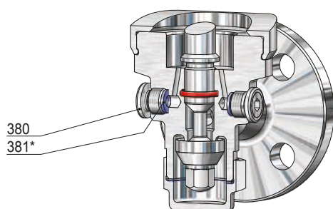
Manometer connection G 1/4
