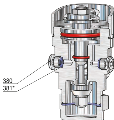
Manometer connection G 1/4
