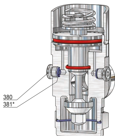
Manometer connection G 1/4
