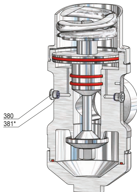
Manometer connection G 1/4
