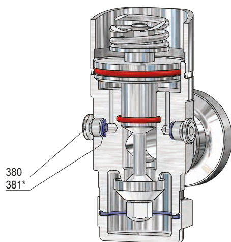
Manometer connection G 1/4
