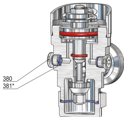
Manometer connection G 1/4
