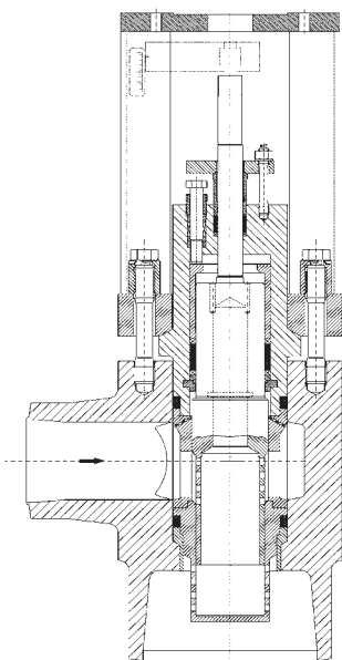
2-stage expansion with balanced pressure for ZK 613
